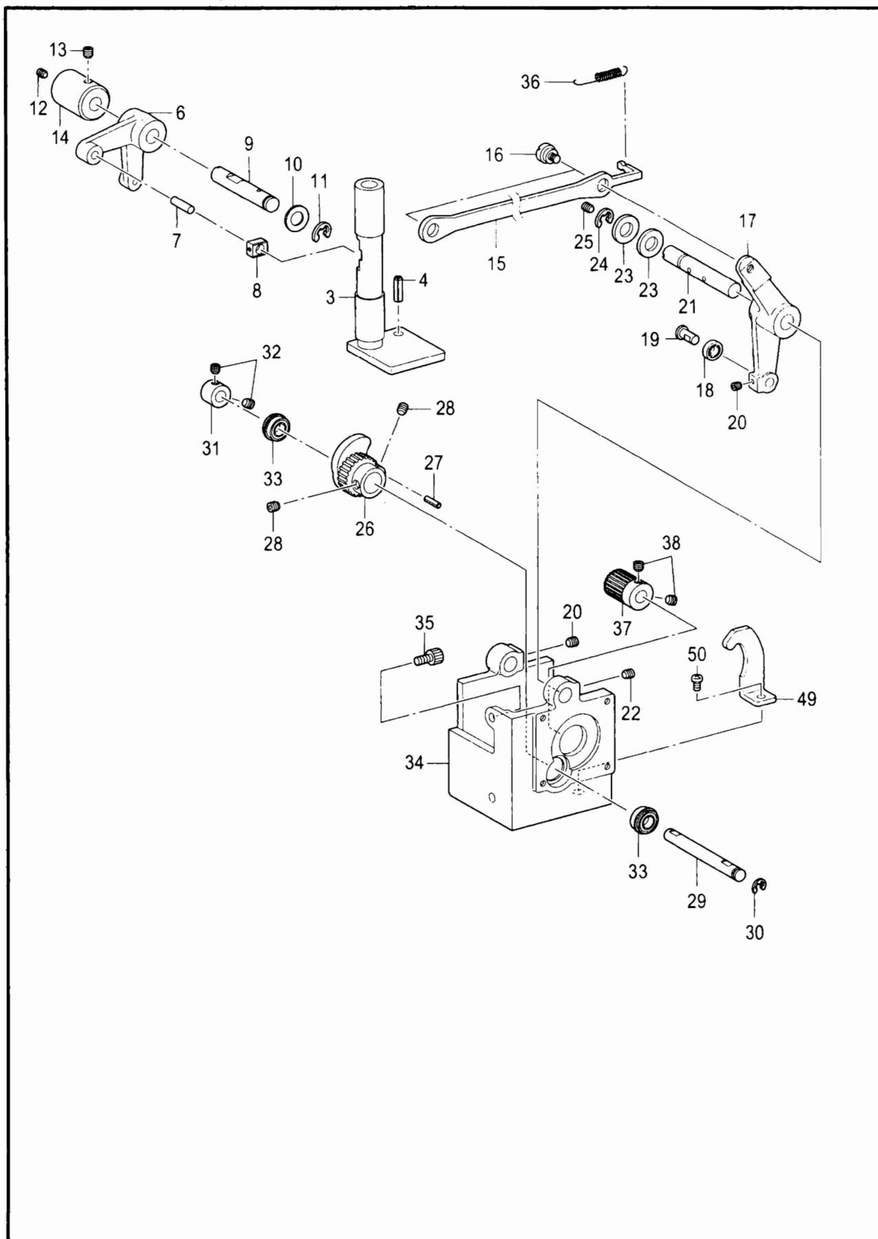
D 1 抬压装置 / Work clamp lifter mechanism
